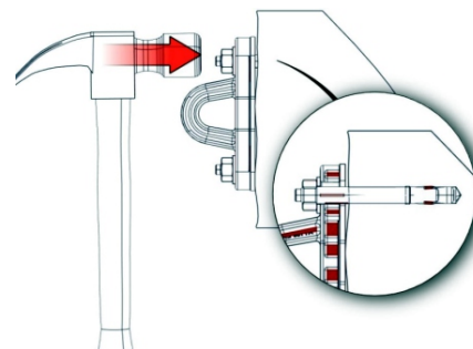
Figure 10. Embedding throughbolts in concrete.
