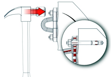
Figure 10. Embedding throughbolts in concrete.
