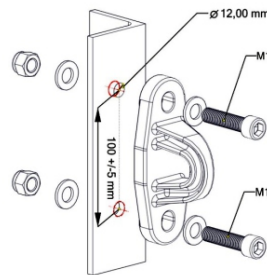
Figure 5. Installation of bolt fasteners with anchor point on steel structure
