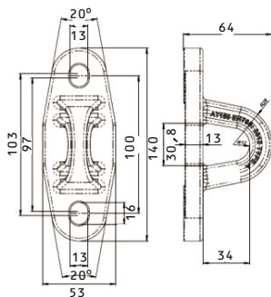
Figure 2. Overall dimensions IRUDEK PRO
