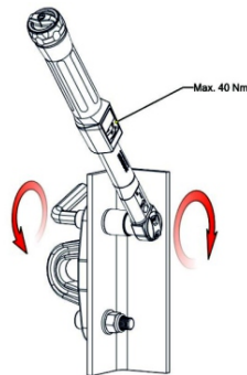
Figure 6. Method of screwing anchor point on steel structure using torque wrench
