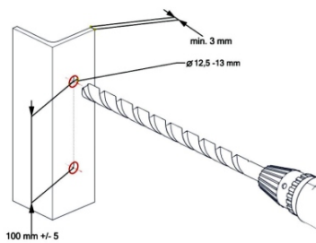
Figure 4. Drilling mounting holes in steel profiles
