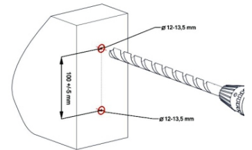
Figure 9. Drilling holes for anchor point IRUDEK PRO 4
